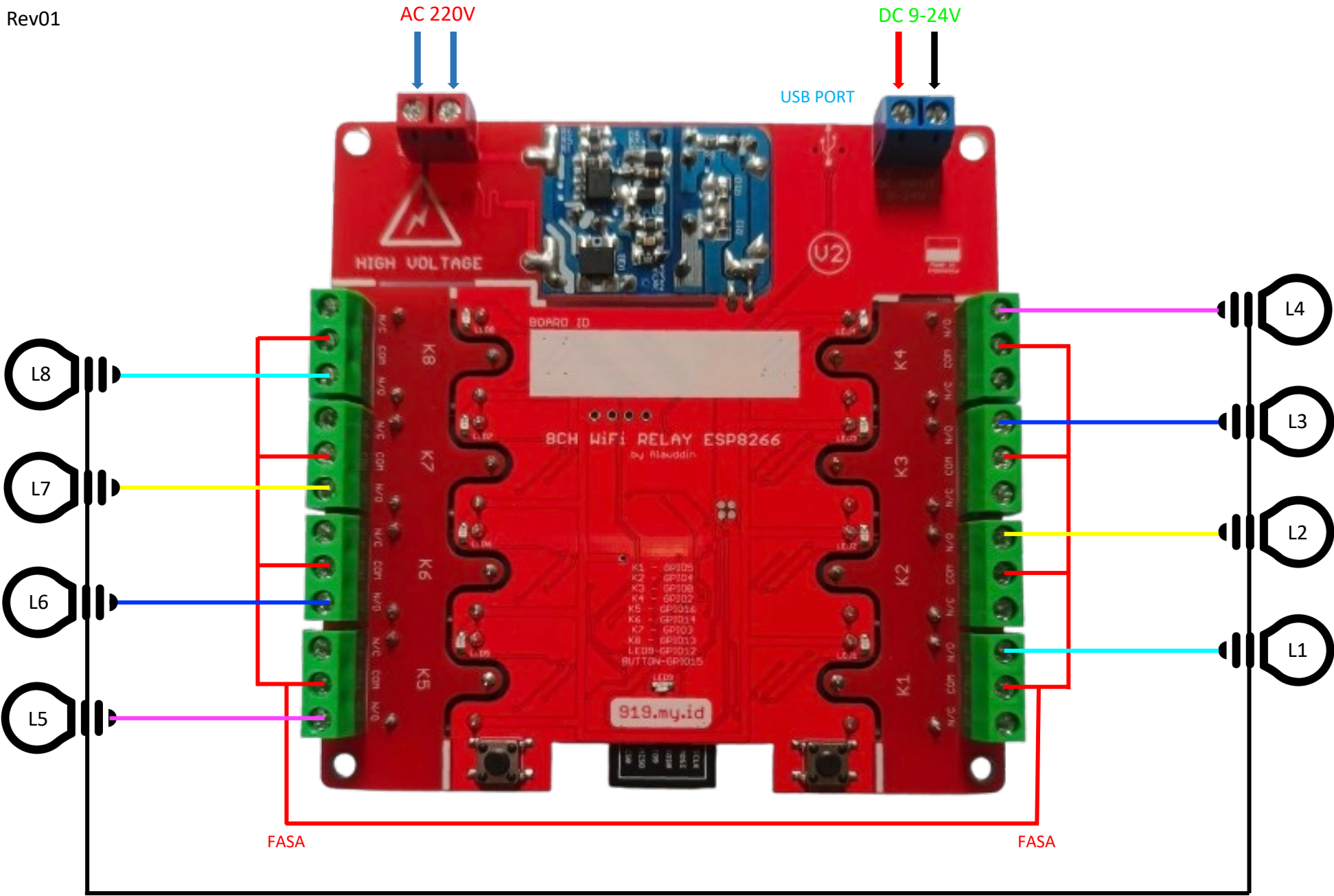
8CH_V2 Board Development Kit ESP8266
